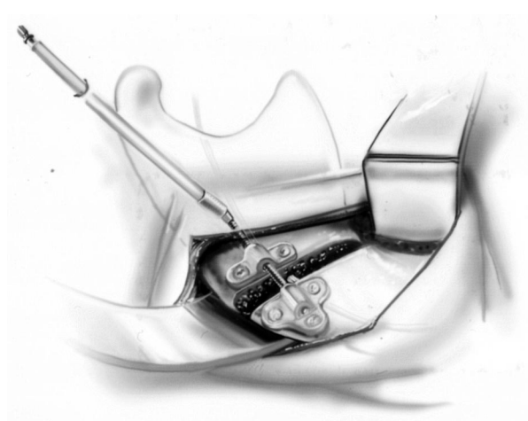
FIG. 3. Activation of the distractor after bilateral osteotomies. Note that the drive screw is fully seated in the distal housing and that osteotomies are complete.
